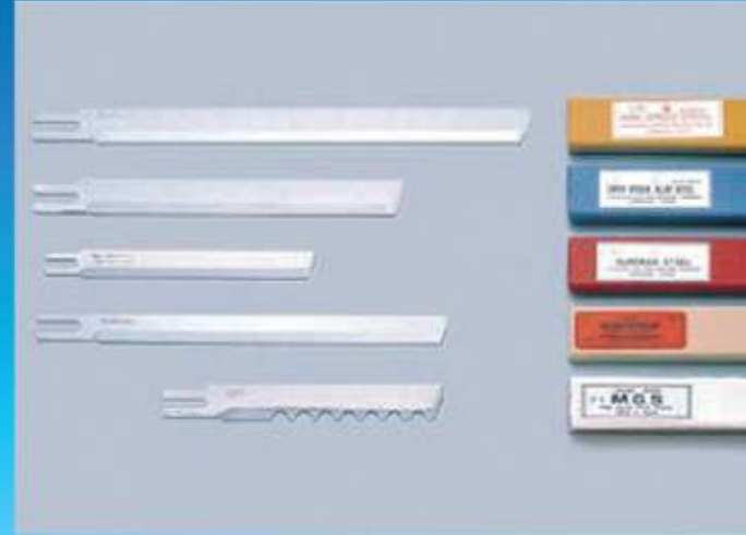
Straight Knives 鋸刃
